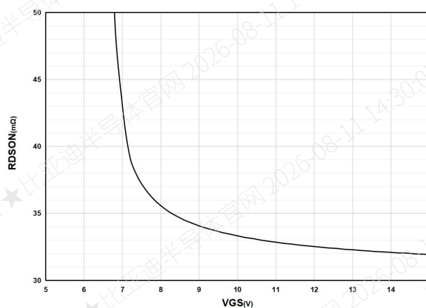
Figure 6. Typical drain-source on-state resistance as a function of gate-source voltage( I_D=32.5\text{A} )
