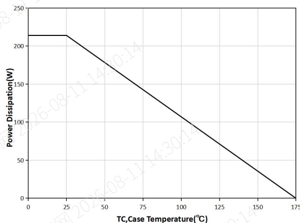
Figure 16. Maximum Power Derating
