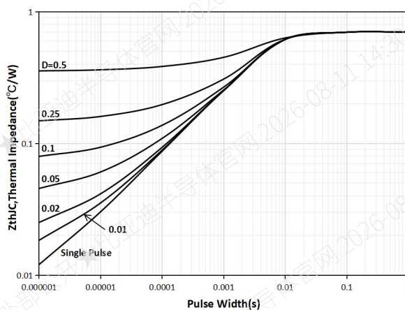
Figure 18. Maximum Transient Thermal Impedance
