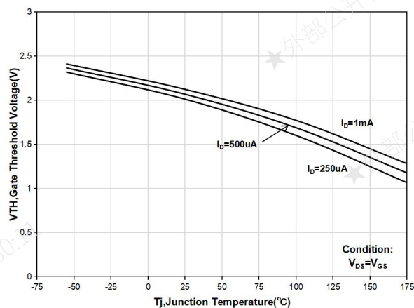
Figure 8. Typical Gate Threshold Voltage vs. Junction Temperature
