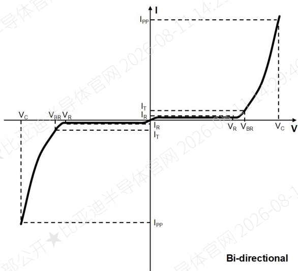
Fig.1 I-V Curve Characteristics
