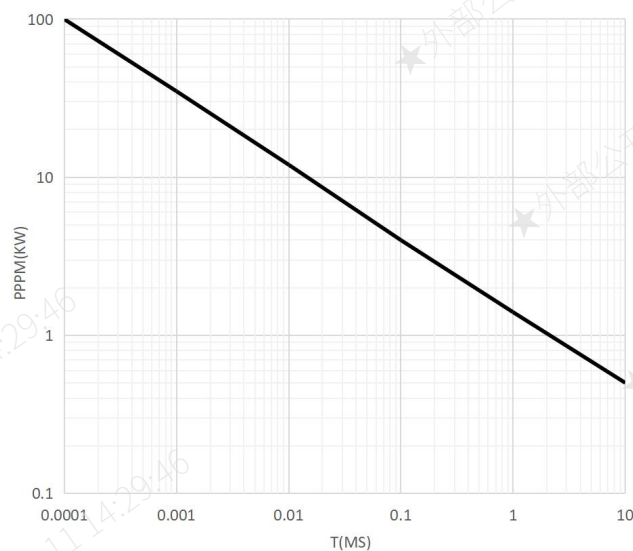
Fig.2 Peak Pulse Power Rating
