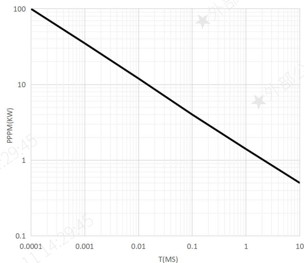
Fig.2 Peak Pulse Power Rating
