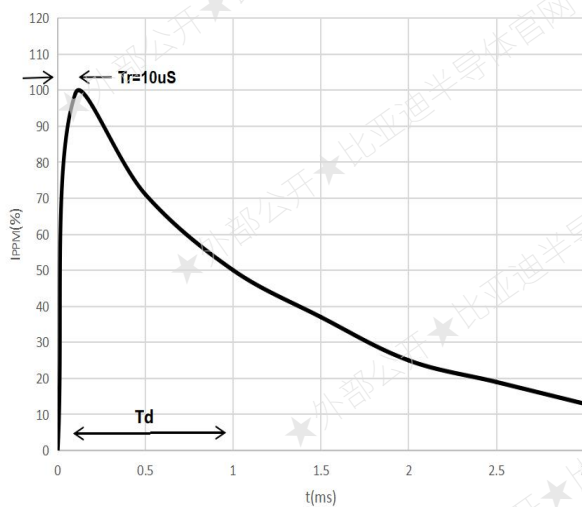
Fig.3 Clamping Power Pulse Waveform
