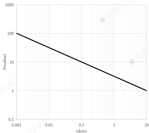
Fig.2 Peak Pulse Power Rating
