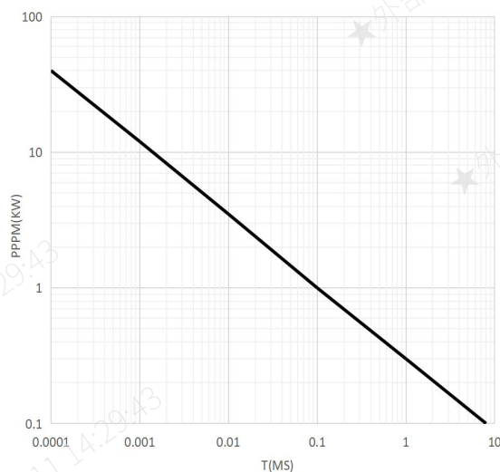
Fig.2 Peak Pulse Power Rating
