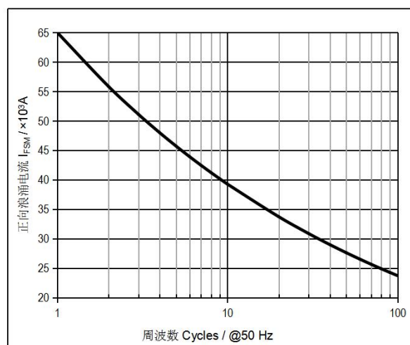
图6. 浪涌电流与周波数的关系曲线 Fig.6 Surge current vs cycles
