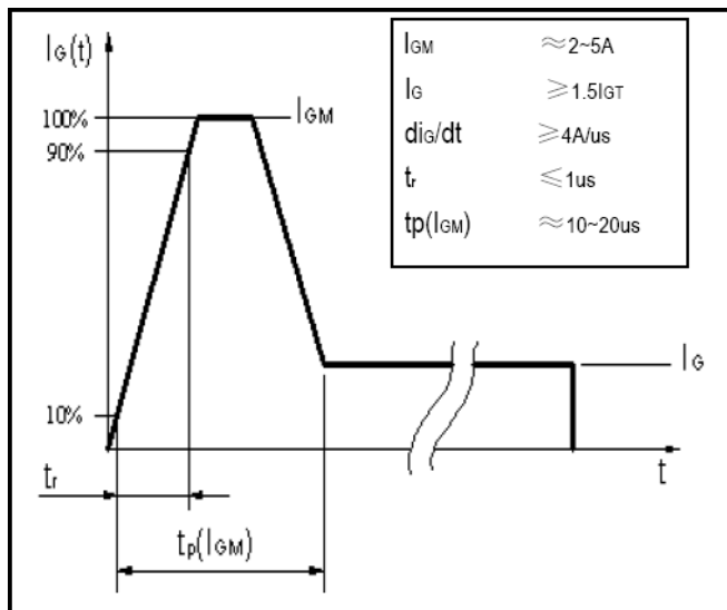
Fig7. Recommended gate current waveform
