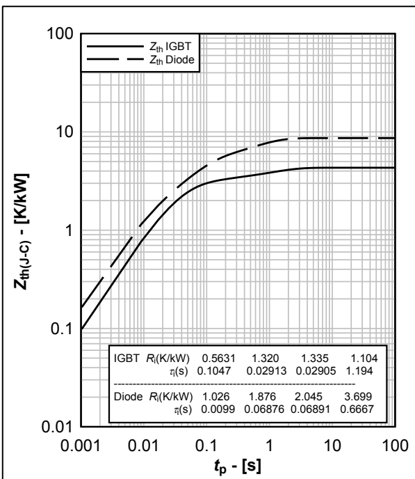
图 10. 瞬态热阻抗曲线, Z_{th(J-C)} = f(t_p)
