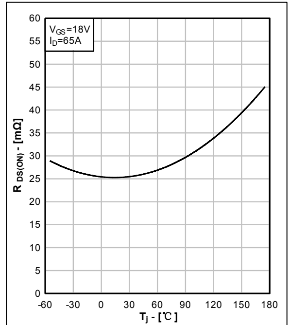
图7. 导通电阻典型曲线, R_{DS(on)} = f(T_J) Fig.7 Typical On-Resistance characteristics, R_{DS(on)} = f(T_J)
