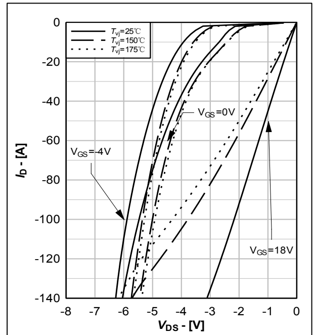
图13. 体二极管及第三象限输出特性典型曲线, I_D = f(V_{DS}) Fig.13 Typical body diode output and 3rd quadrant characteristic, I_D = f(V_{DS})
