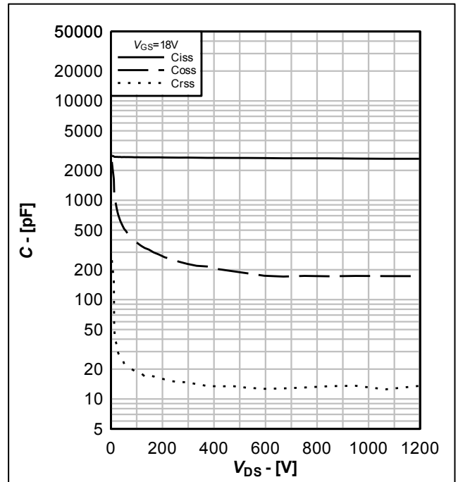
图11. 电容特性典型曲线, C = f(V_{DS}) Fig.11 Typical capacity characteristic, C = f(V_{DS})
