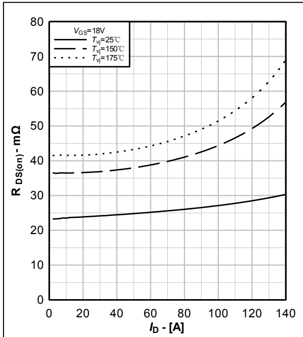
图6. 导通电阻典型曲线, R_{DS(on)} = f(I_D) Fig.6 Typical On-Resistance characteristics, R_{DS(on)} = f(I_D)
