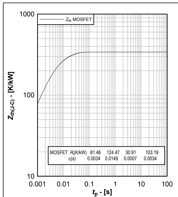
图14. 瞬态热阻抗曲线, Z_{th(J-C)} = f(t_p) Fig.14 Transient thermal impedance, Z_{th(J-C)} = f(t_p)
