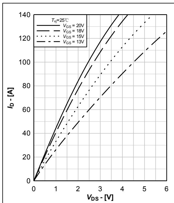
图2. 输出特性典型曲线, I_D = f(V_{DS}) , T_{vj} = 25\text{ }^{\circ}\text{C} Fig.2 Typical output characteristics, I_D = f(V_{DS}) , T_{vj} = 25\text{ }^{\circ}\text{C}
