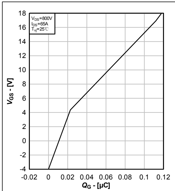
图12. 栅极电荷特性典型曲线, V_{GS} = f(Q_G) Fig.12 Typical gate charge characteristic, V_{GS} = f(Q_G)
