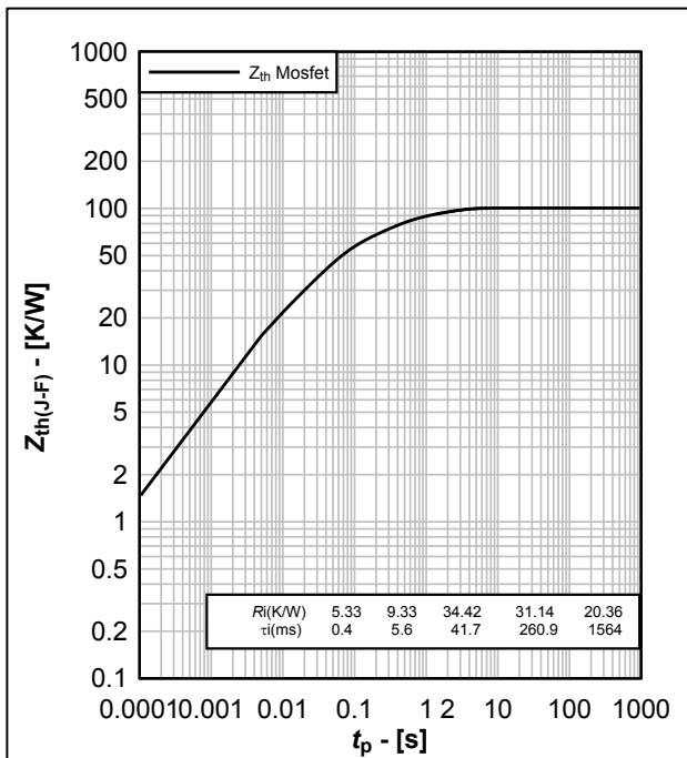
图 17. 瞬态热阻抗曲线, Z_{th(J-F)} = f(t_p)
