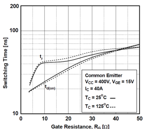
Figure 7. Turn-On Characteristics vs. Gate Resistance
