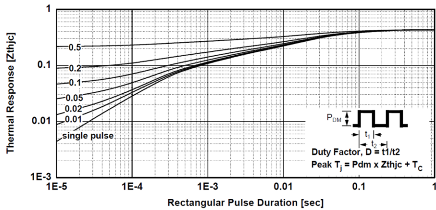
Figure 15. Transient Thermal Impedance of IGBT
