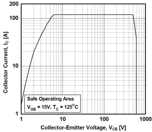
Figure 13. Turn off Switch SOA Characteristics
