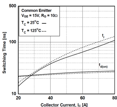
Figure 10. Turn-On Characteristics vs. Collector Current
