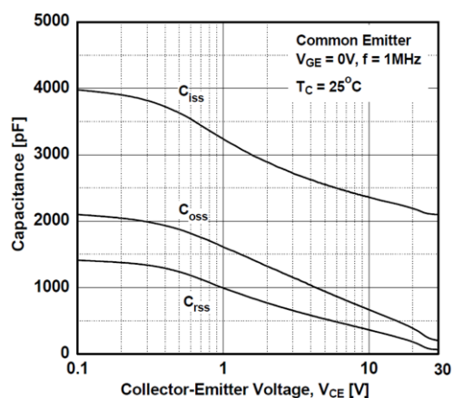
Figure 6. Capacitance Characteristics
