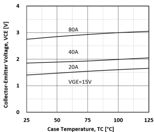
Figure 3. Saturation Voltage vs. Case Temperature
