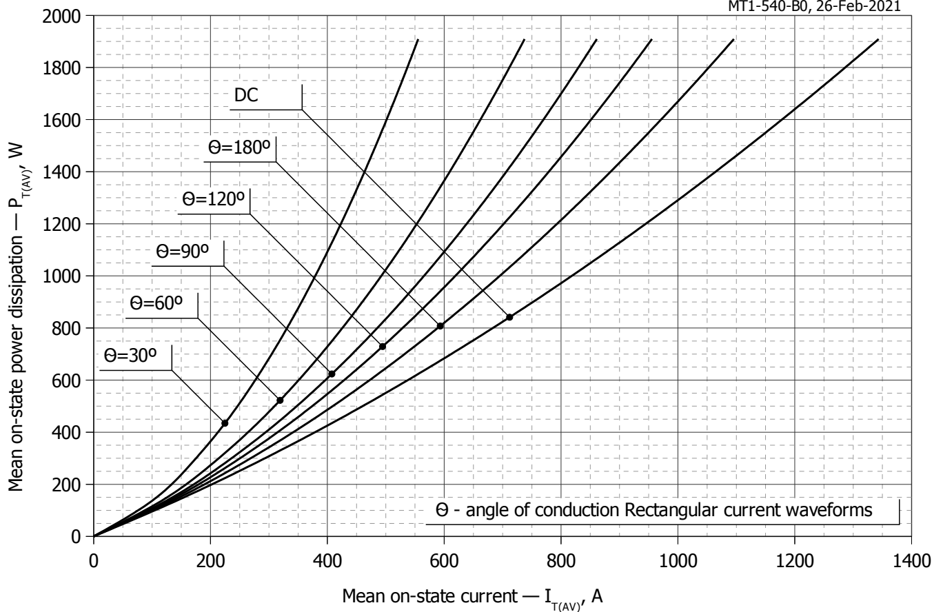
Fig. 7 – Mean on-state power dissipation P_{TAV} vs. mean on-state current I_{TAV} for rectangular current waveforms at different conduction angles and for DC ( f=50\text{Hz} , DSC)
