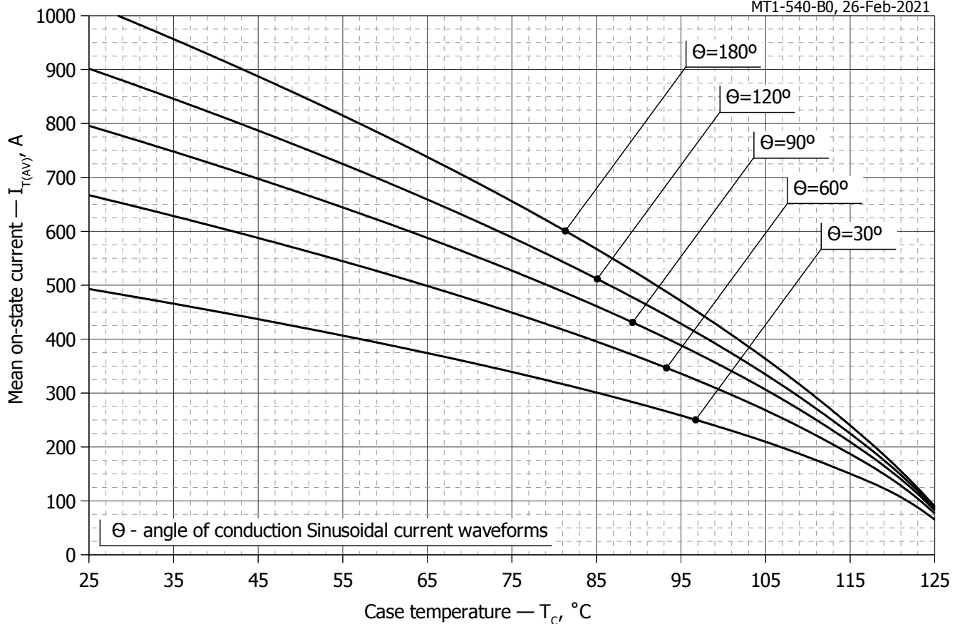
Fig. 8 – Mean on-state current I_{TAV} vs. case temperature T_c for sinusoidal current waveforms at different conduction angles ( f=50\text{Hz} , DSC)
