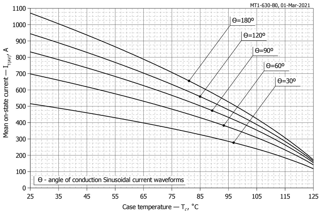
Fig. 8 – Mean on-state current I_{TAV} vs. case temperature T_c for sinusoidal current waveforms at different conduction angles ( f=50\text{Hz} , DSC)
