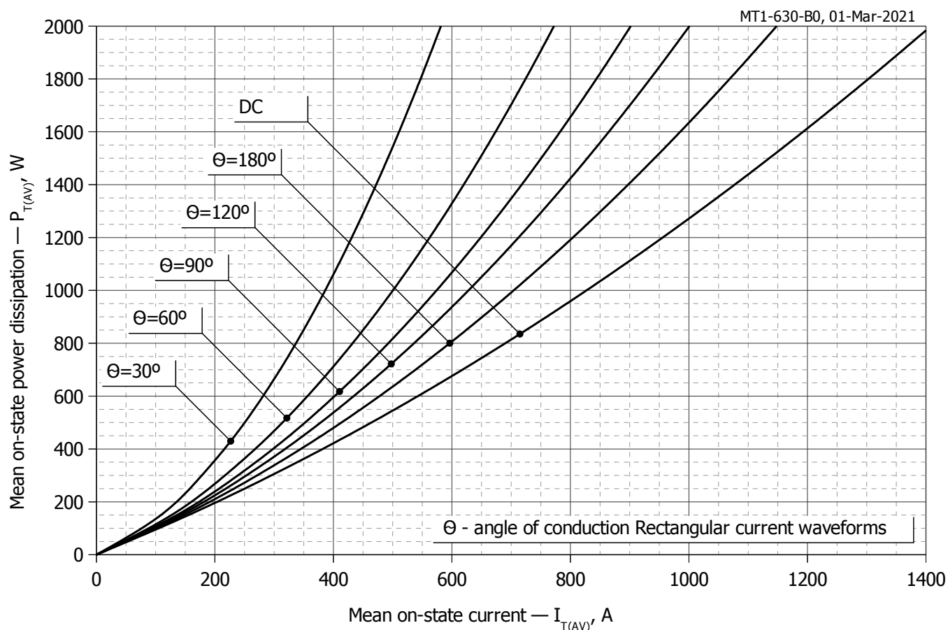
Fig. 7 – Mean on-state power dissipation P_{TAV} vs. mean on-state current I_{TAV} for rectangular current waveforms at different conduction angles and for DC ( f=50\text{Hz} , DSC)
