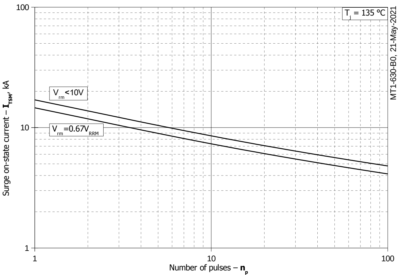
Fig. 11 - Maximum surge on-state current I_{TSM} vs. number of pulses n_p
