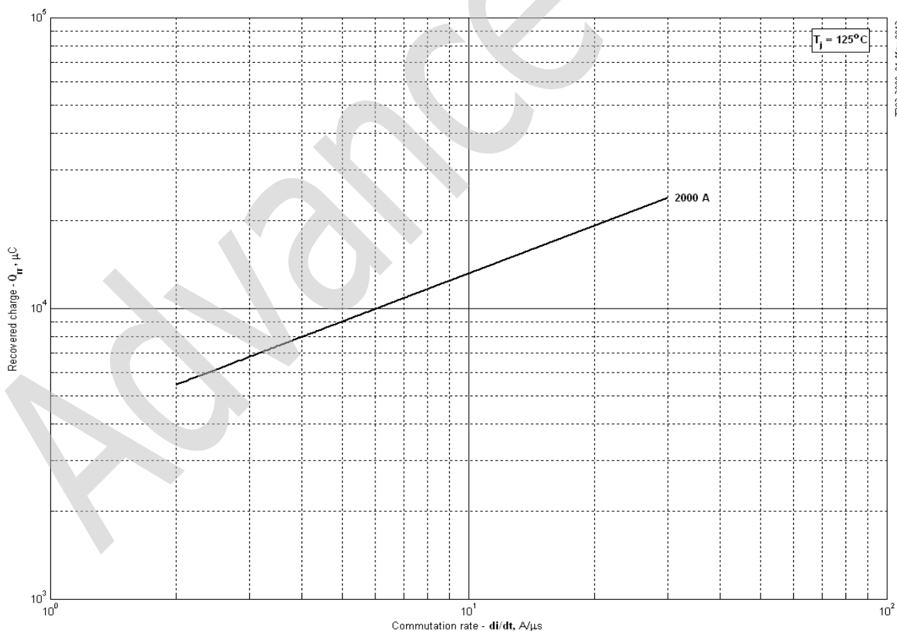
Fig 6 – Maximum recovered charge Q_{rr} vs. commutation rate di_R/dt (25% chord)
