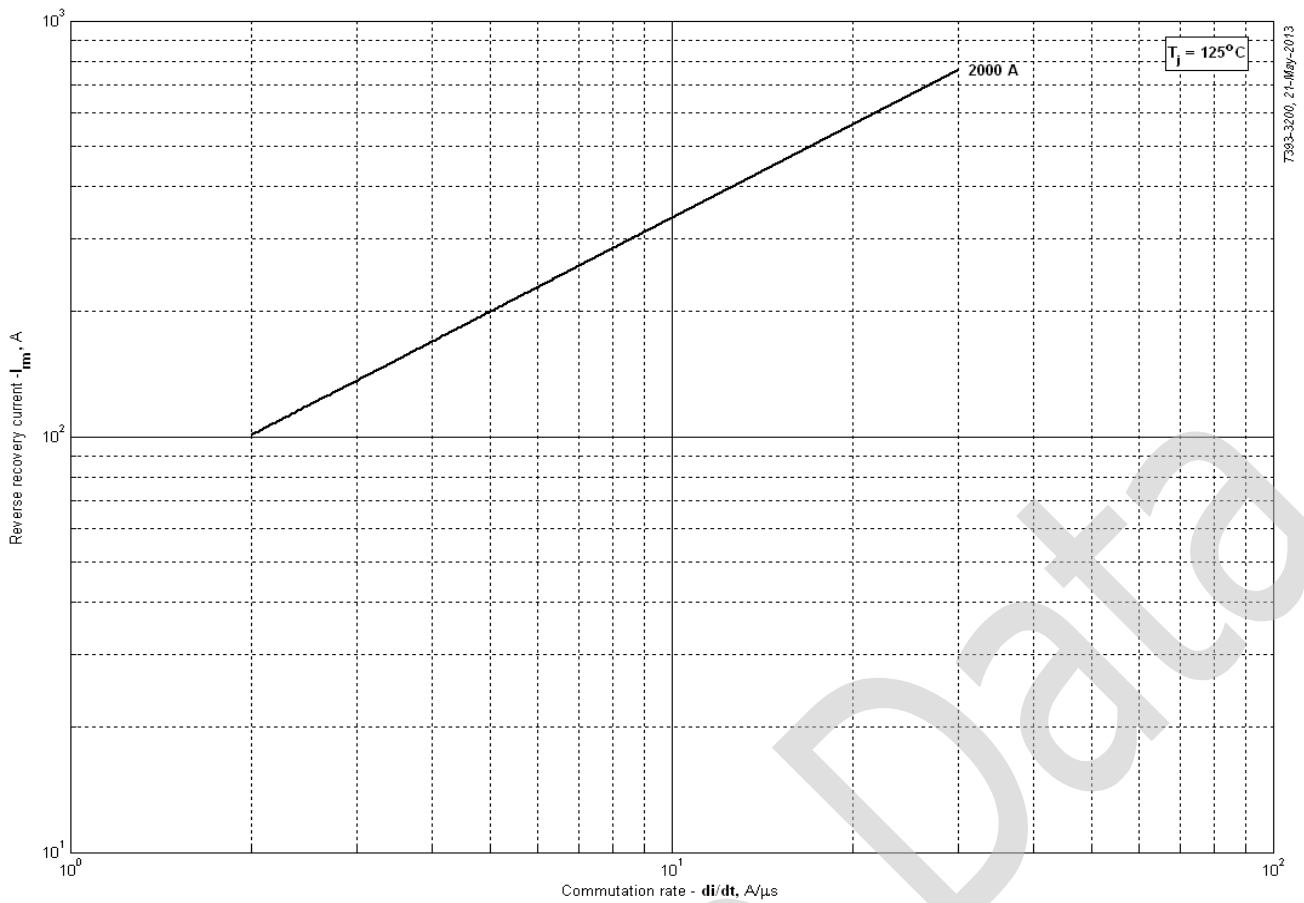
Fig 7 – Maximum reverse recovery current I_{rr} vs. commutation rate di_R/dt
