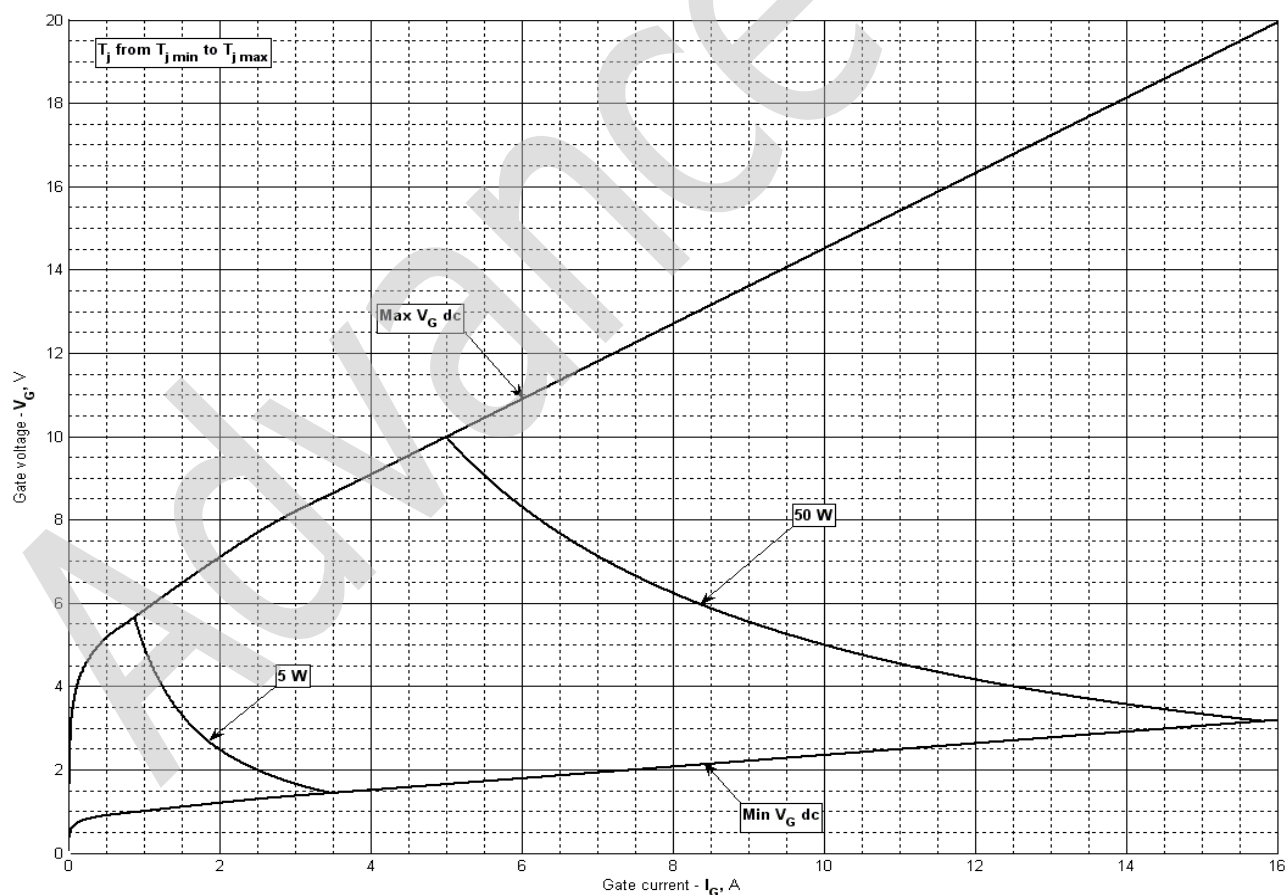
Fig 4 - Gate characteristics – Power curves
