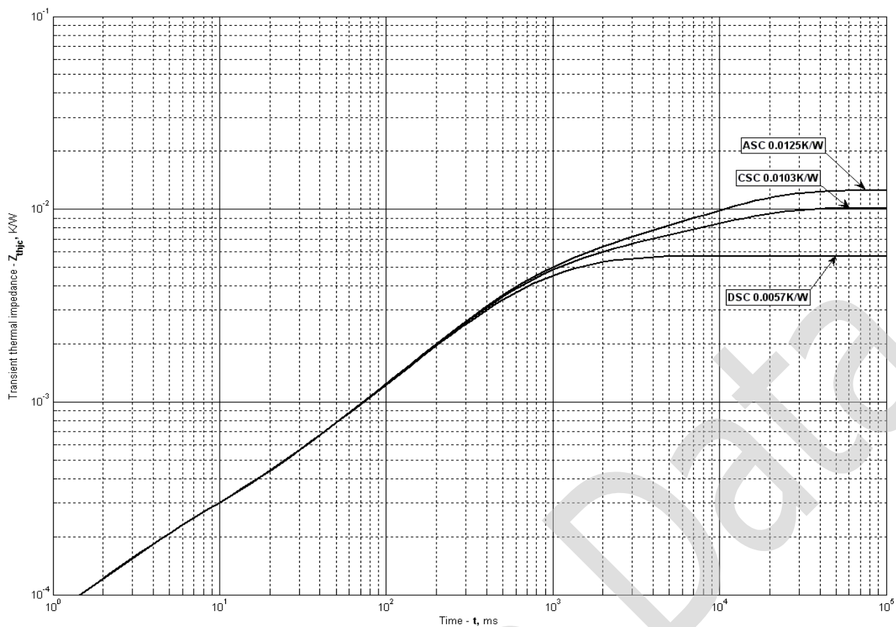
Fig 2 – Transient thermal impedance Z_{thjc} vs. time t
