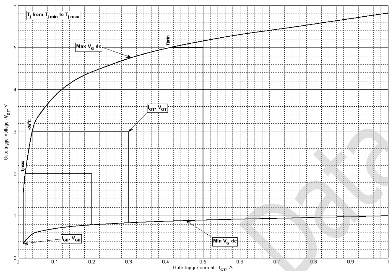
Fig 3 – Gate characteristics – Trigger limits
