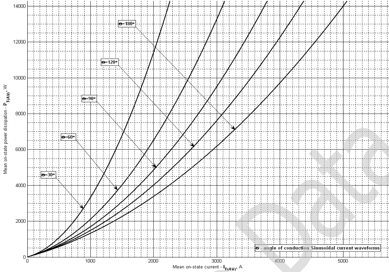
Fig. 9 - Mean on-state power dissipation P_{TAV} vs. mean on-state current I_{TAV} for sinusoidal current waveforms at different conduction angles ( f=50\text{Hz} , DSC)
