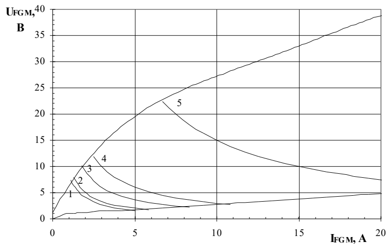
Fig. 1 On-state characteristics of typical device
