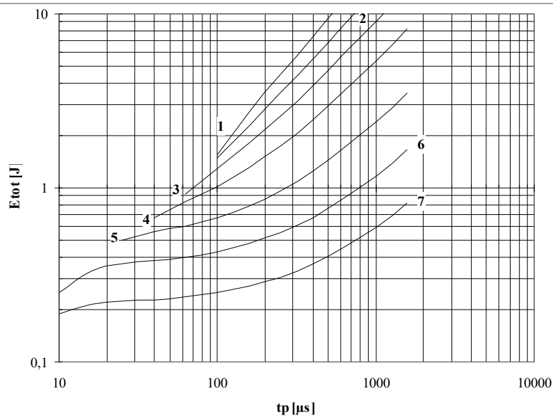
Fig. 26 Square wave energy per pulse
