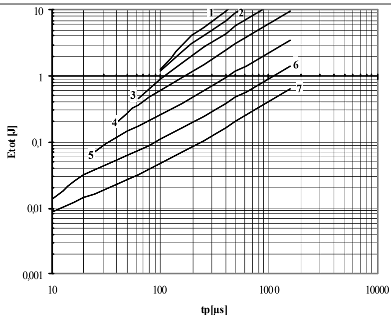
Fig. 24 Square wave loss energy per pulse
