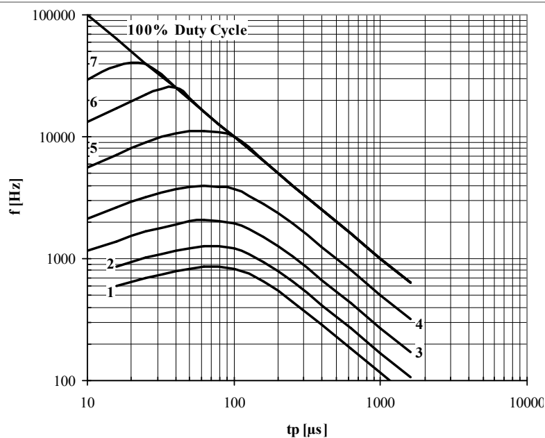
Fig. 12 Sine wave frequency ratings
