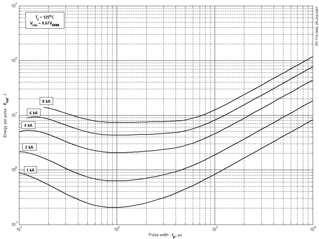
Fig 9 – Sine wave energy per pulse
