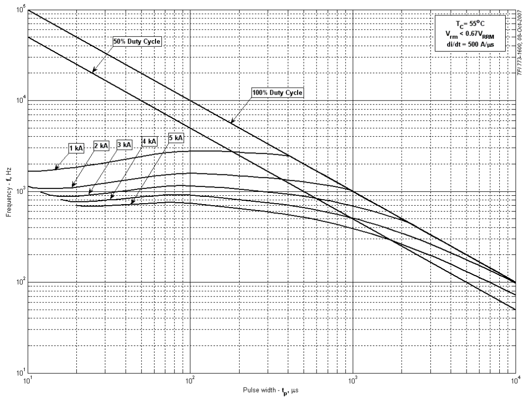
Fig 21 – Square wave frequency ratings
