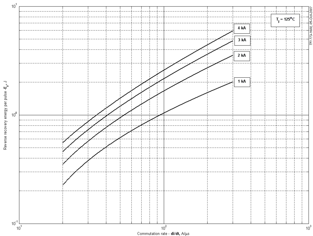
Fig 7 – Reverse recovery energy per pulse
