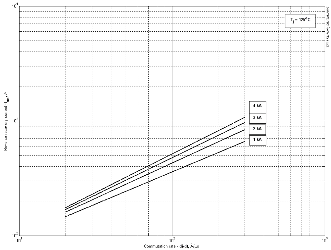
Fig 5 – Peak reverse recovery current, I_{rr}
