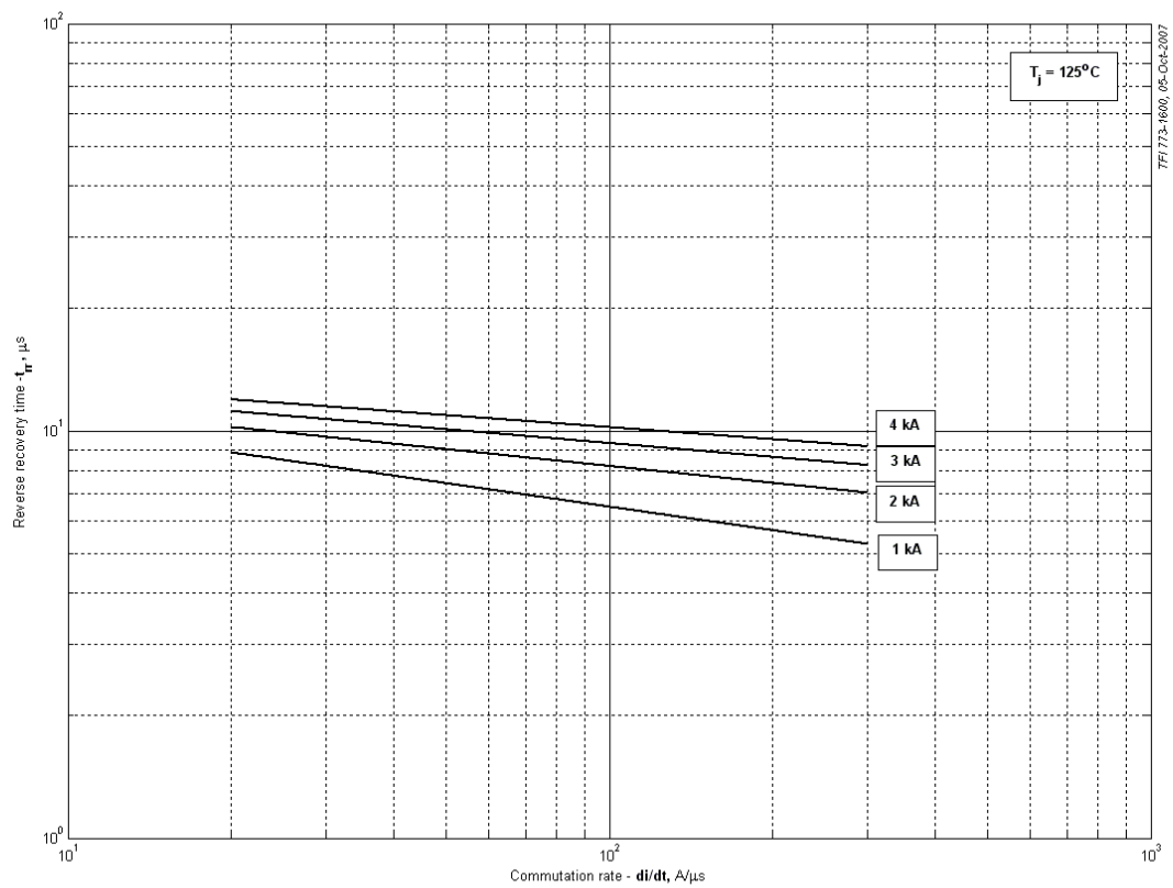
Fig 6 – Maximum recovery time, t_{rr} (50% chord)
