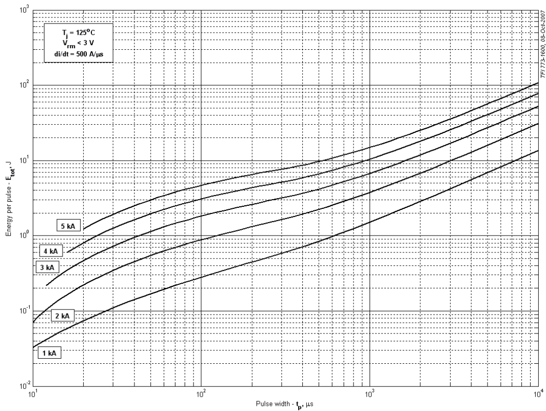
Fig 19 – Square wave energy per pulse
