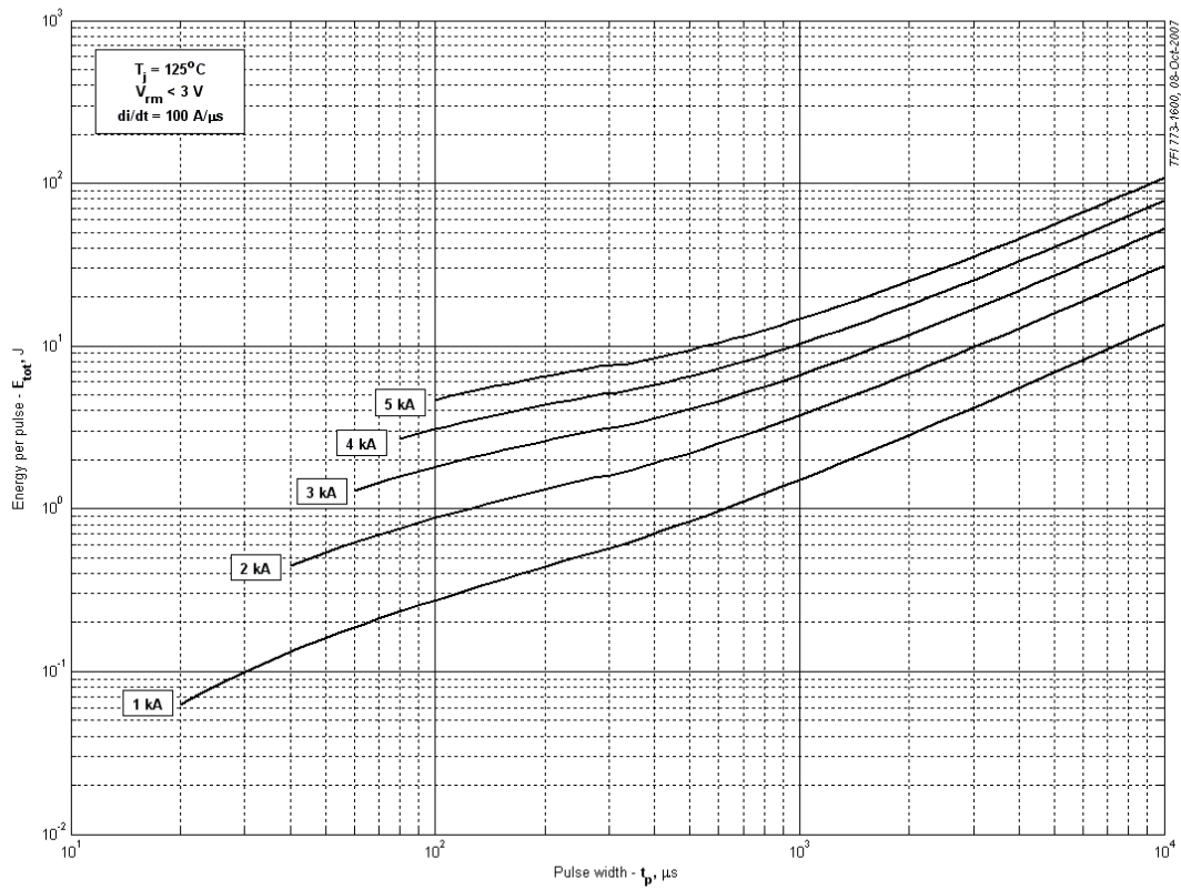
Fig 18 – Square wave energy per pulse
