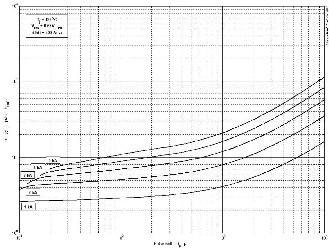
Fig 25 – Square wave energy per pulse
