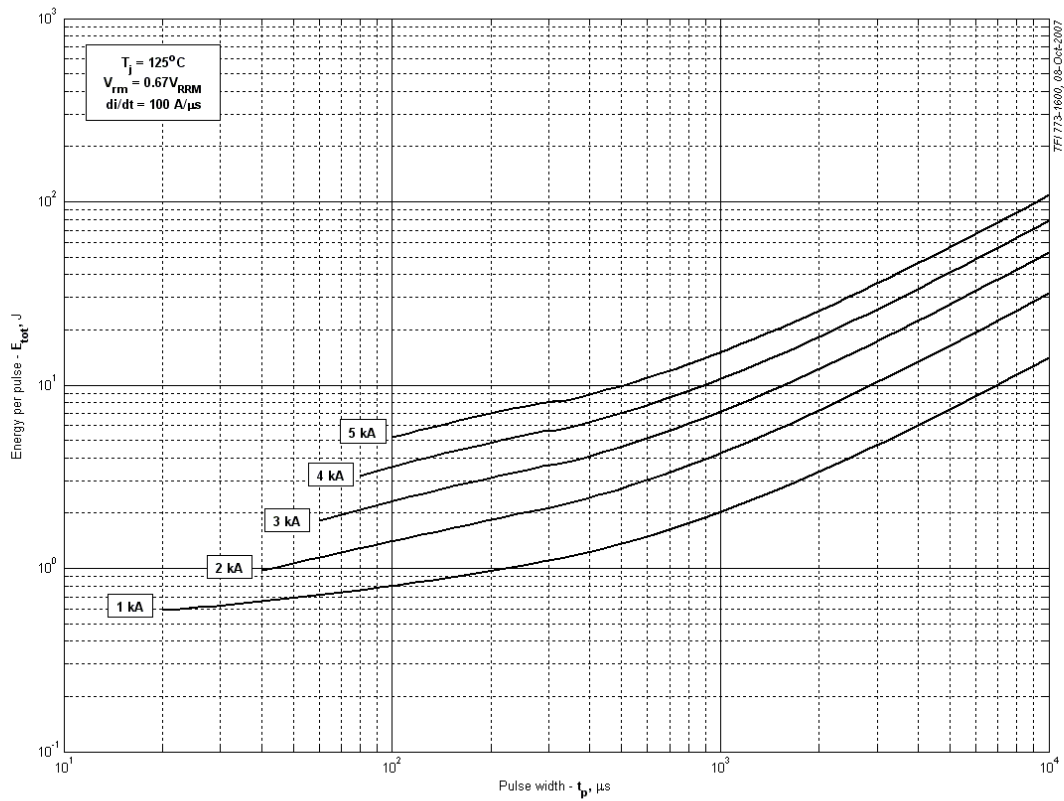
Fig 24 – Square wave energy per pulse
