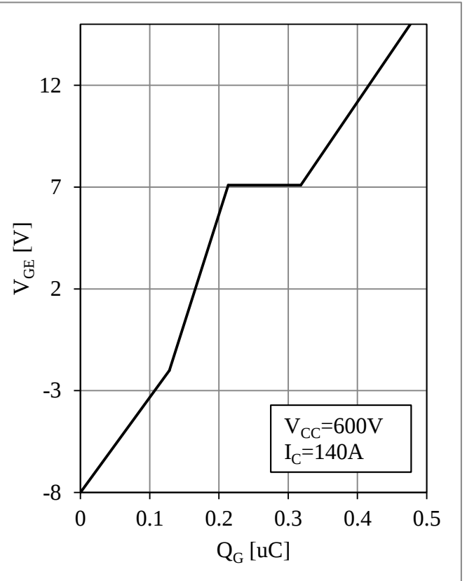
Fig 12. IGBT Gate Charge vs. V_{CE}
