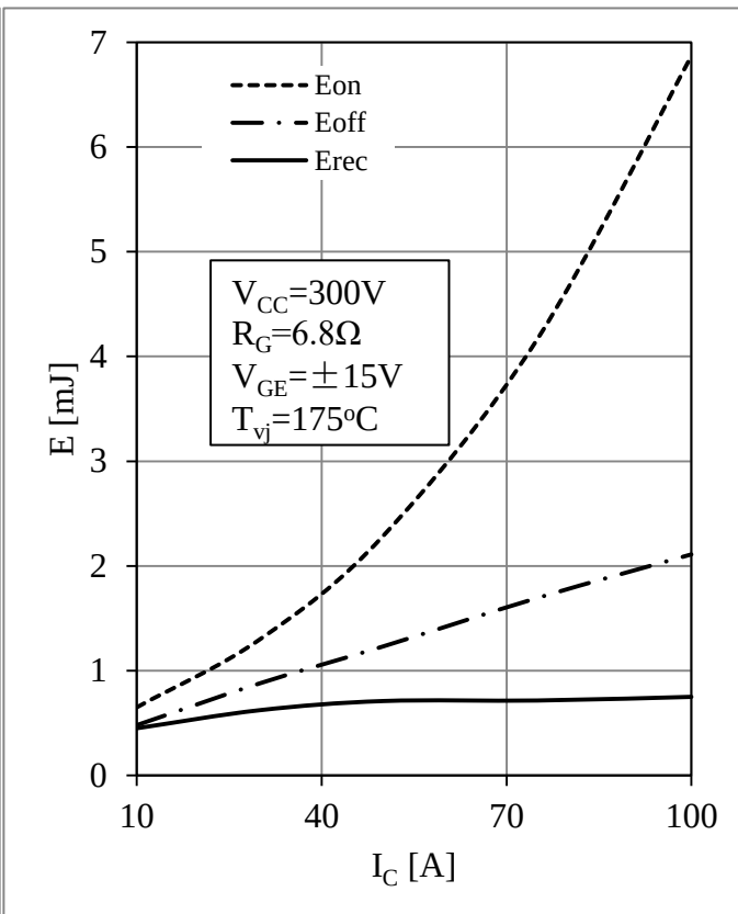
Fig 8. Switching Energy Loss vs. I_C
