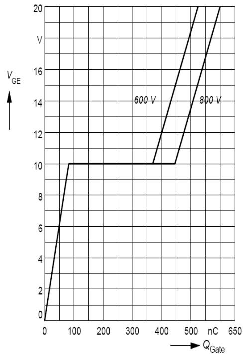
Fig 5. Gate Charge Characteristics.
