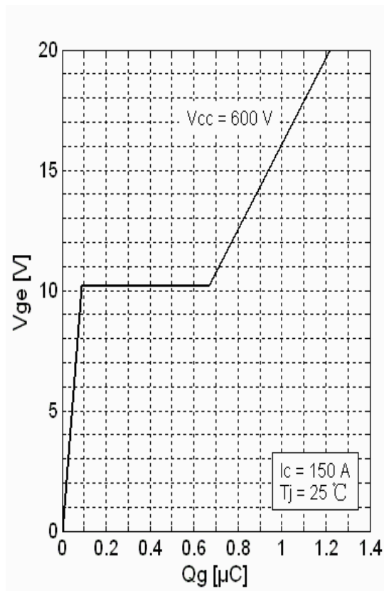
Fig 5. Gate Charge Characteristics.
