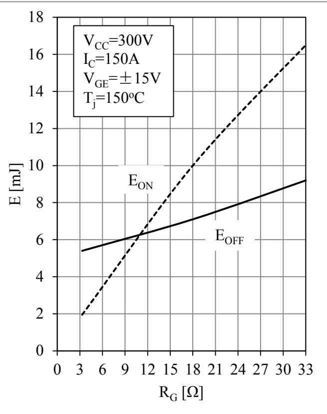
Fig 4. T1-T4 IGBT Switching Loss vs. R_G
