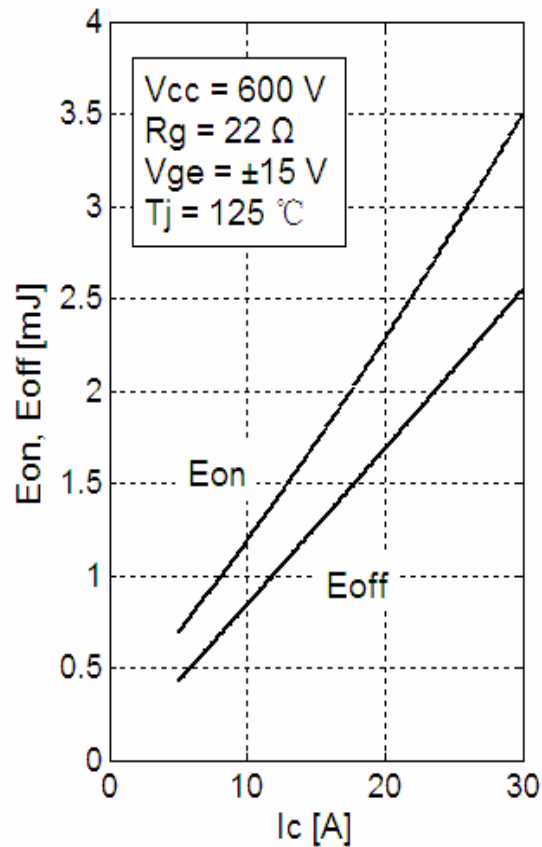
Fig 3. IGBT-inverter Switching Loss vs. I_c
