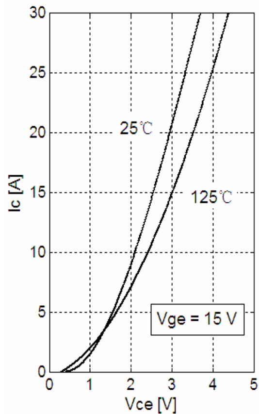
Fig 12. IGBT-brake Output Characteristics
