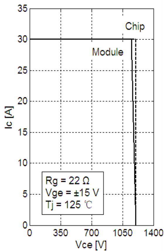
Fig 5. IGBT-inverter RBSOA
