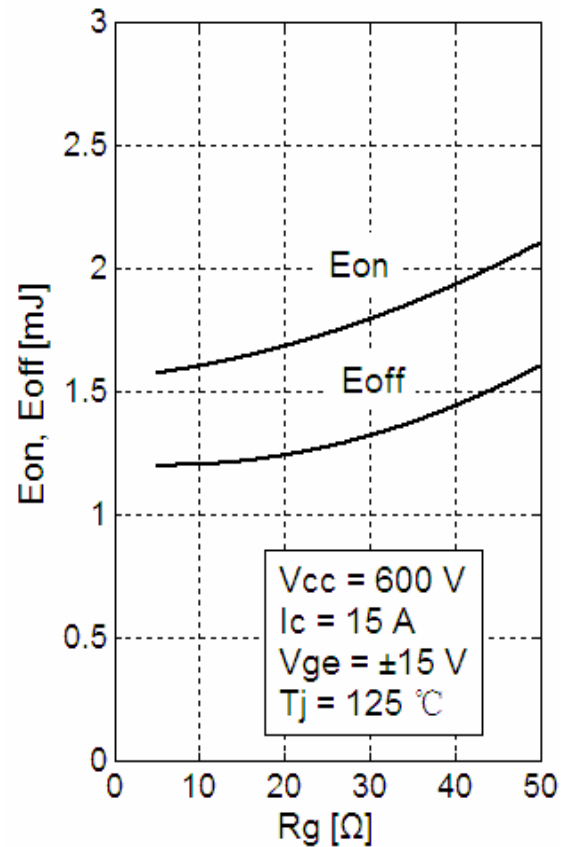
Fig 4. IGBT-inverter Switching Loss vs. R_g
