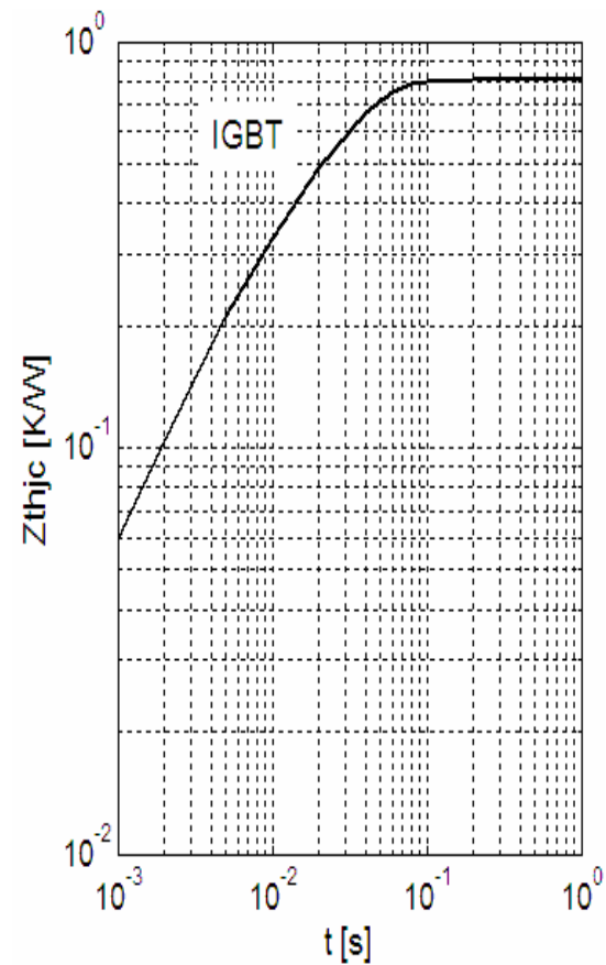
Fig 6. IGBT-inverter Transient Thermal Impedance
