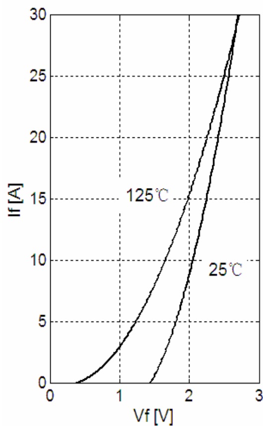
Fig 7. Diode-inverter Forward Characteristics
