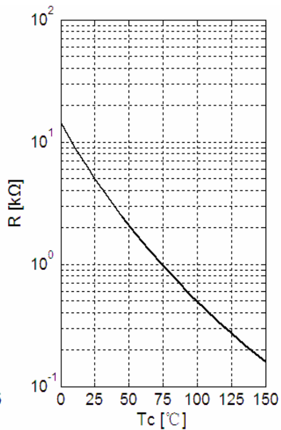
Fig 14. NTC-Temperature Characteristic
