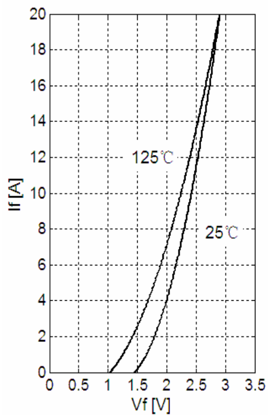
Fig 13. Diode-brake Forward Characteristics
