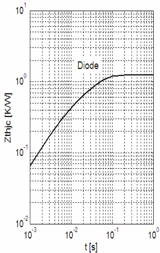
Fig 10. Diode-inverter Transient Thermal Impedance
