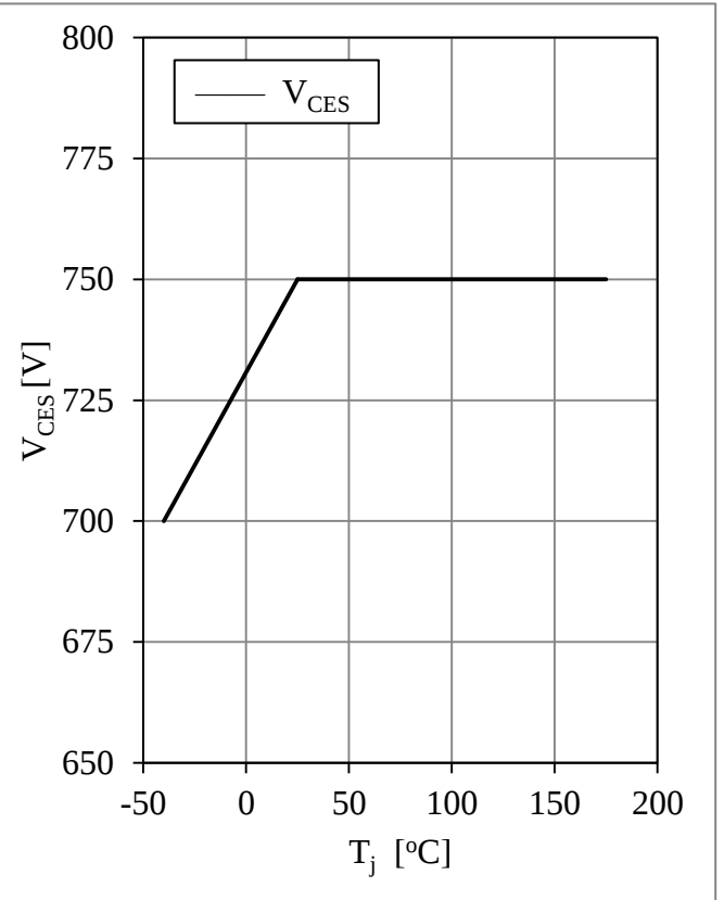
Fig 16. Maximum Allowed Collector-Emitter Voltage
