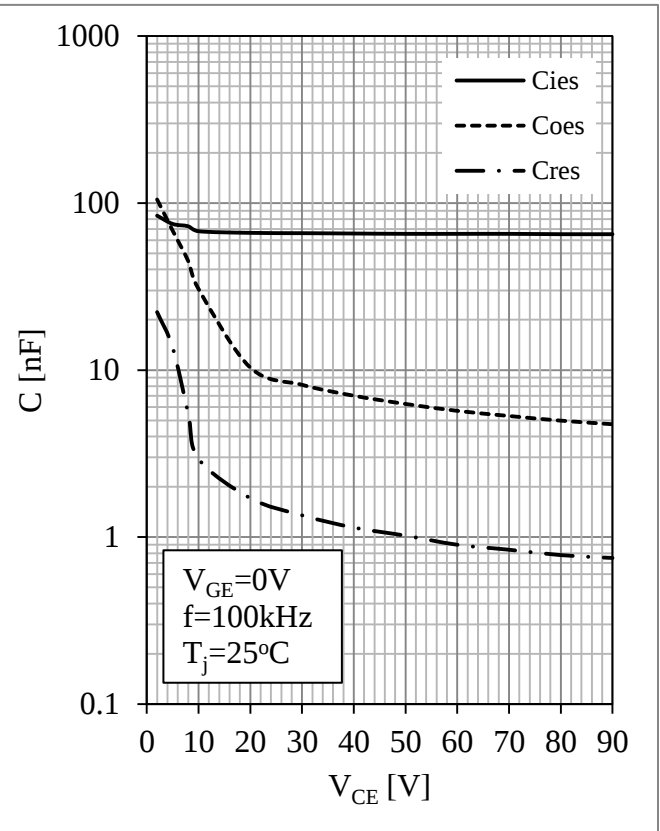
Fig 14. IGBT Capacity Characteristic
