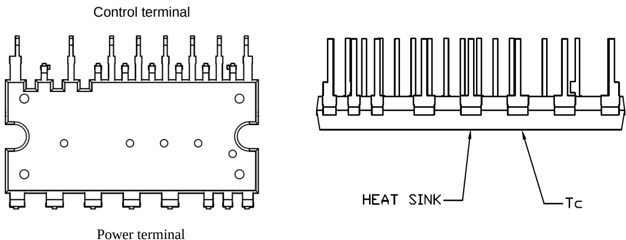
Figure 4. T_c Measurement Point
