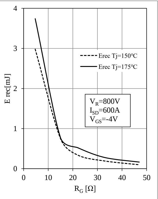
Fig 8. Body Diode Switching Loss vs. R_G
