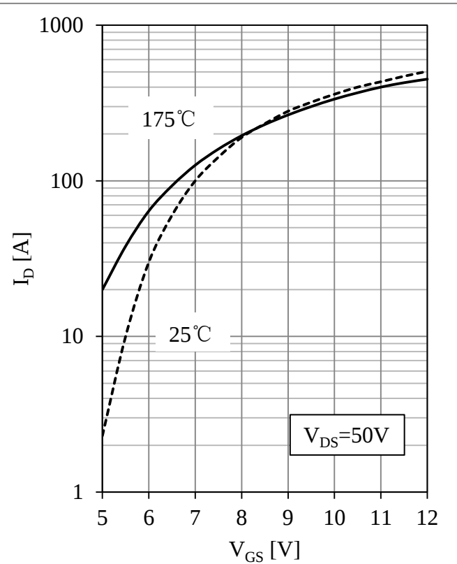
Fig 2. Mosfet Transfer Characteristic
