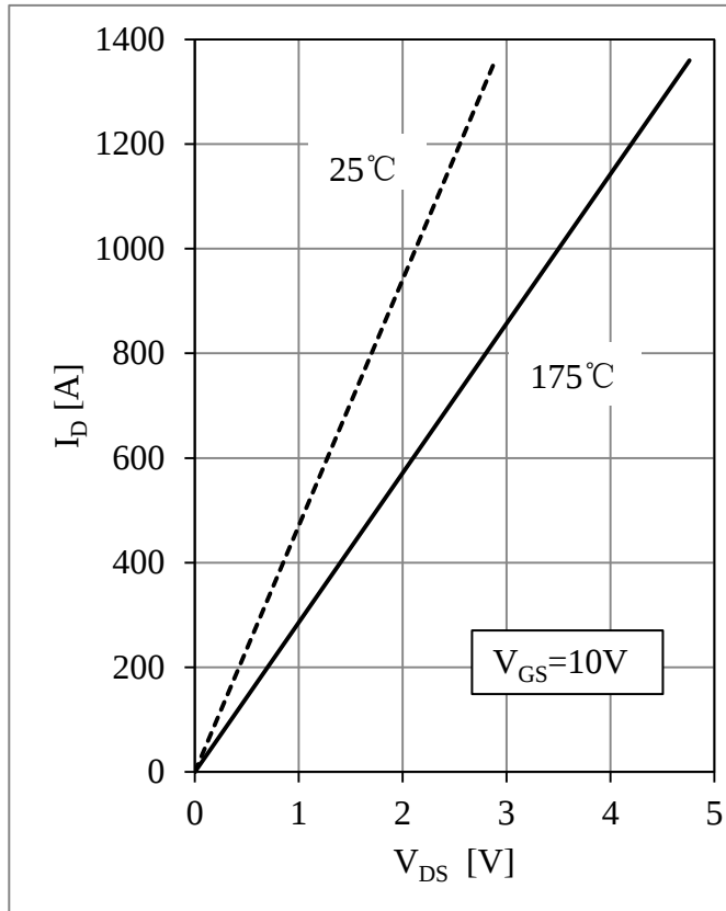
Fig 1. Mosfet Output Characteristic
