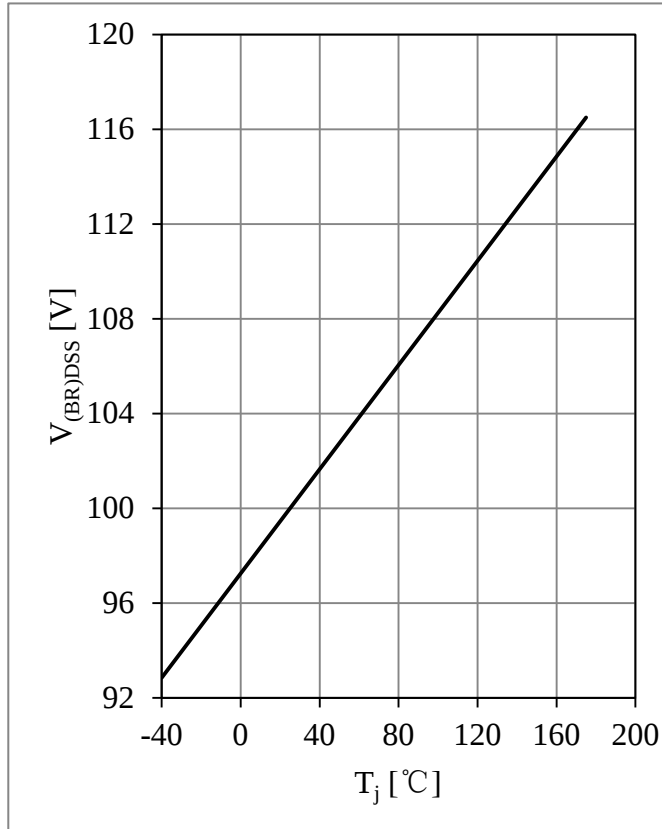
Fig 3. Brakedown Voltage vs. Temperature
