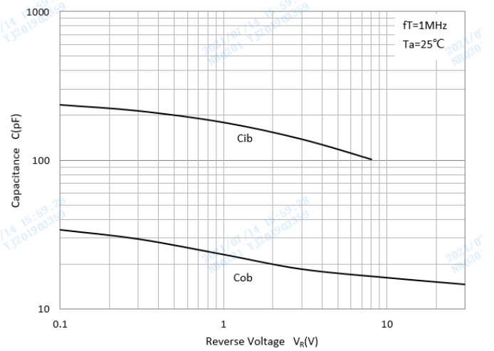
C_{ob}/C_{ib}-V_{CB}/V_{EB}
