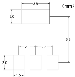
SOT-223-3L Suggested Pad Layout
