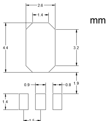
SOT-89 Suggested Pad Layout
