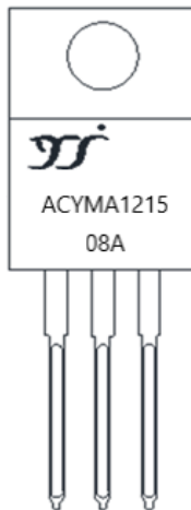
(TO-220AB-1 Package)
