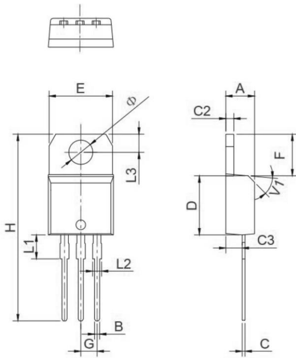
TO-220AB-1
