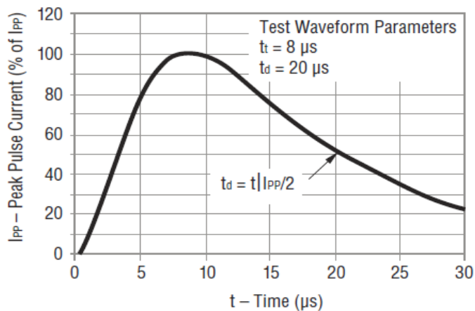
FIG.3 Current 8/20us Waveform per IEC 6100-4-5
