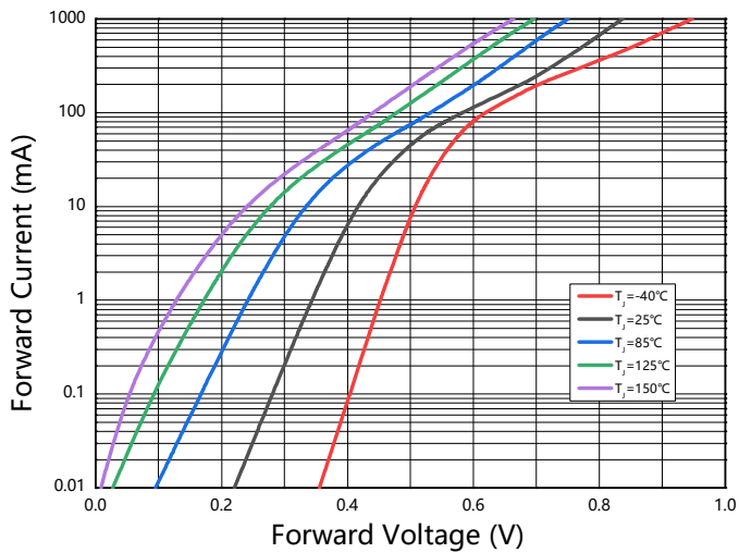
Fig.3: Forward Characteristics
