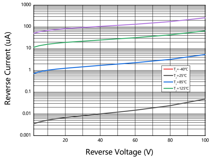
Fig.4: Reverse Characteristics
