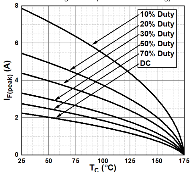
Figure 7. Current Derating
