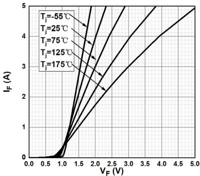
Figure 1. Forward Characteristics
