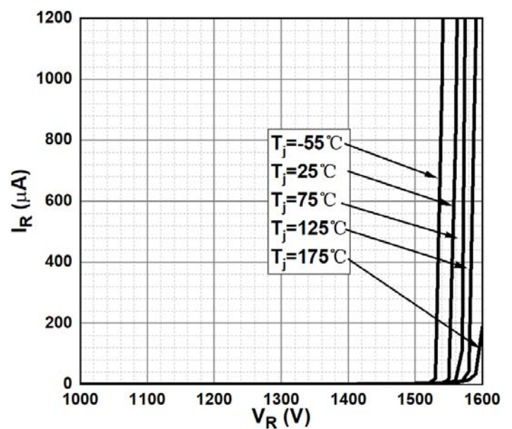
Figure 2. Reverse Characteristics
