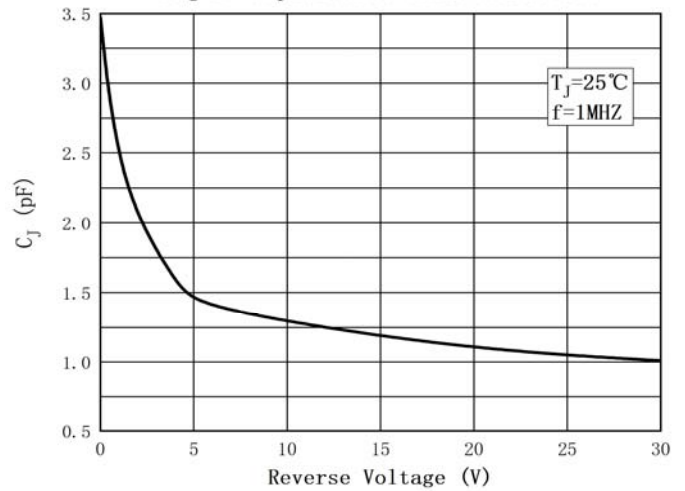
Fig.2: Capacitance Characteristics
