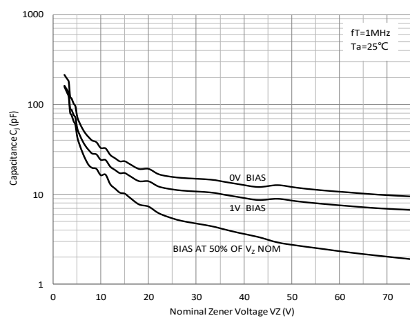
Fig 10: Typical Capacitance
