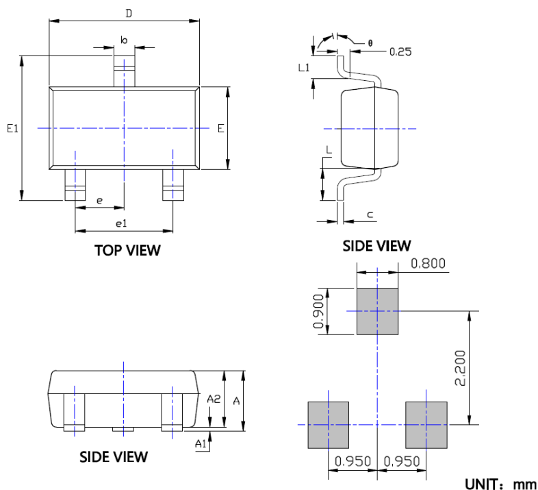
SUGGESTED SOLDER PAD LAYOUT
