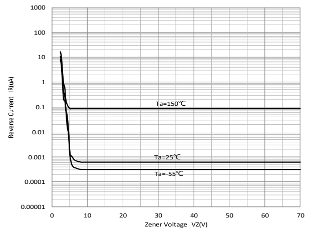
Fig 10: Typical Reverse Current
