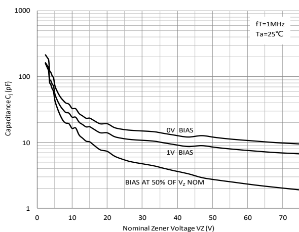
Fig 11: Typical Capacitance
