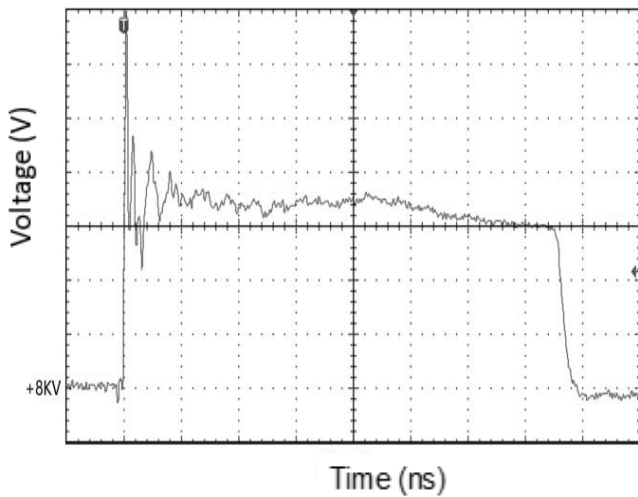
Fig.7 ESD clamping
