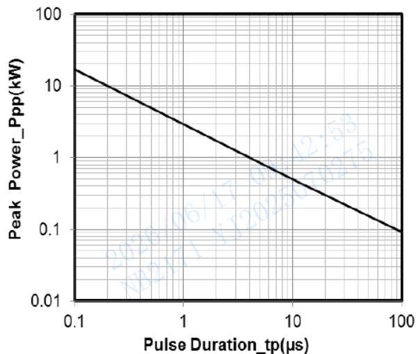
Fig.5 Non-repetitive peak pulse power vs. Pulse time
