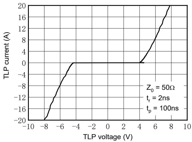
Fig. 9 TLP Measurment
