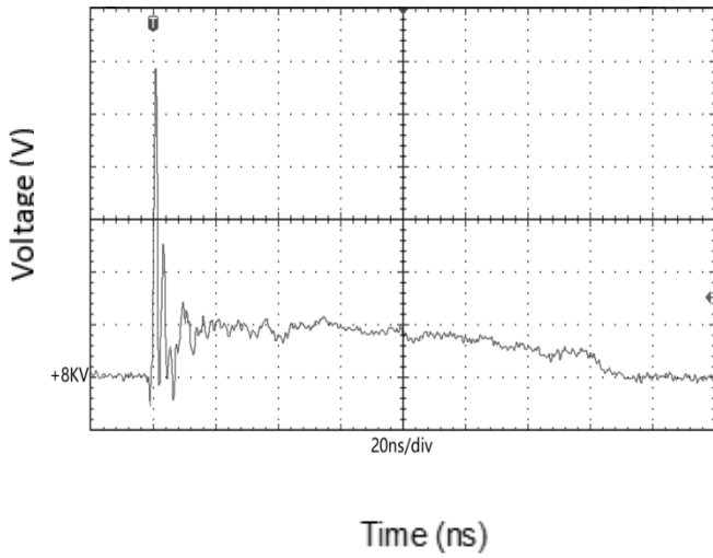
Fig.7 ESD clamping
