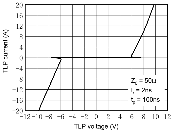
Fig.9 TLP Measurment
