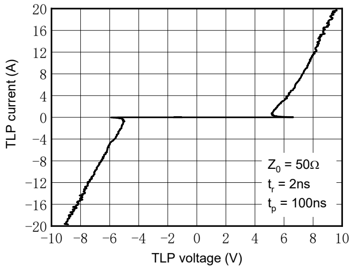
Fig.9 TLP Measurment
