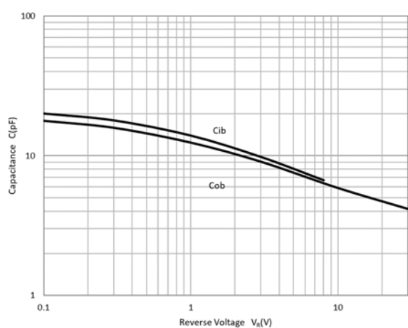
Fig 6: Cob/Cib- V_{CB}/V_{EB}
