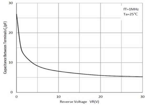
Fig 2: Capacitance Capability
