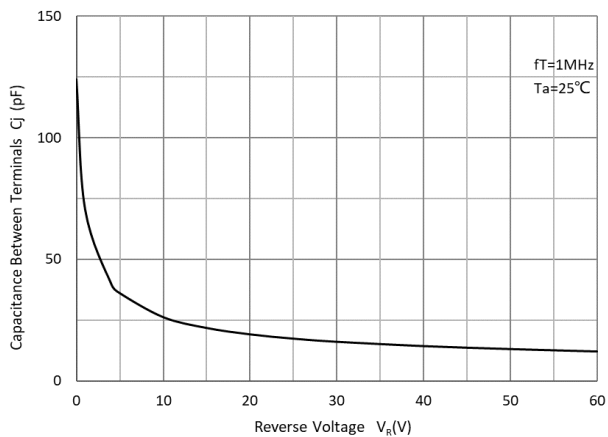
Fig 3: Capacitance Capability
