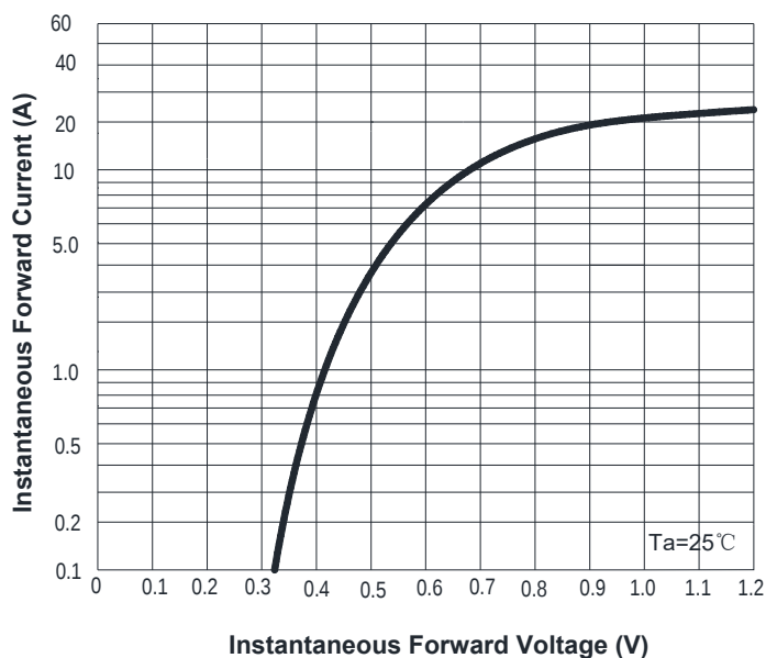
FIG3: Forward Voltage
